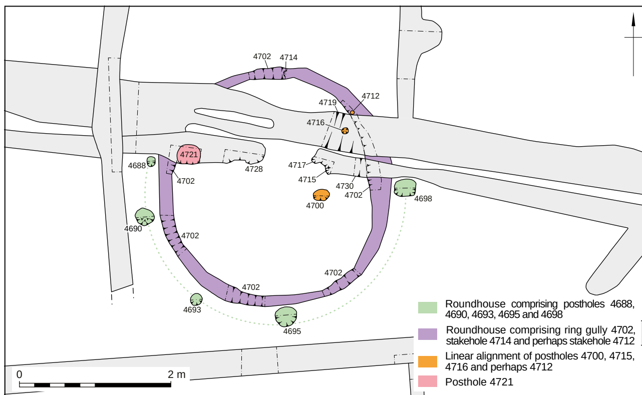
Figure 2.14 Westfield Farm plan of roundhouse 1
