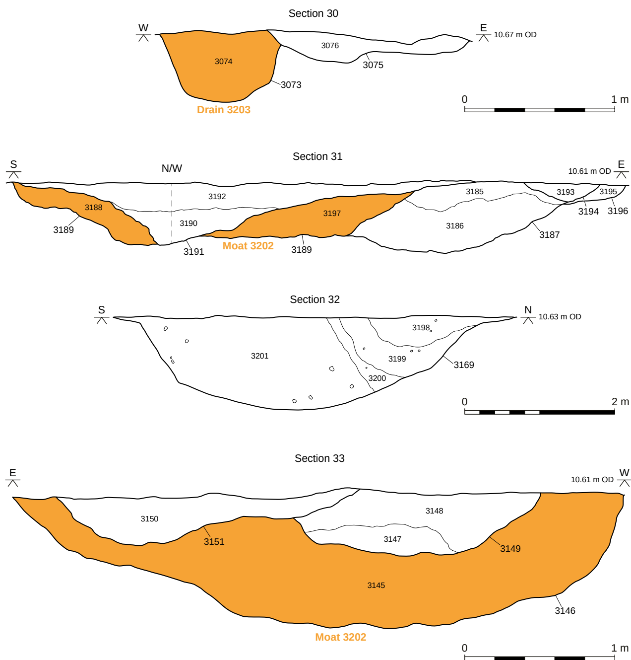
Figure 3.20 Habrough sections
