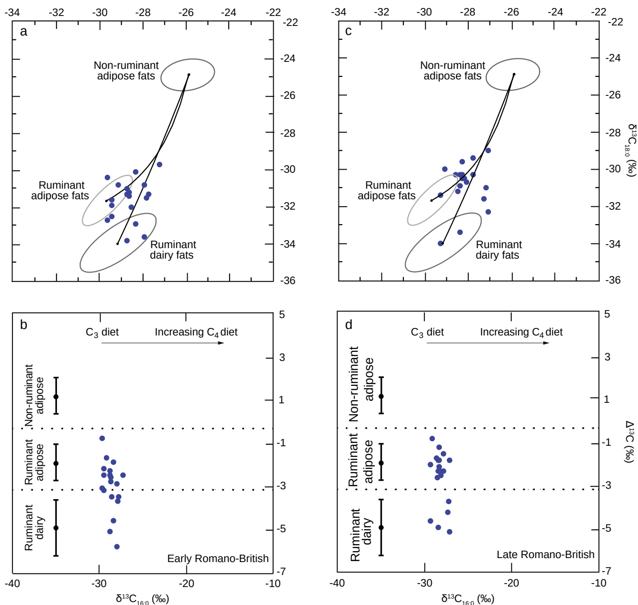
Figure 4.12 Graphs showing \delta^{13}C and \Delta^{13}C values for the C_{16:0} and C_{18:0} fatty acids from early and late Romano-British ceramics
